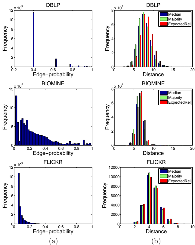
Figure 4: Distribution of (a) edge probabilities, (b) distances.
