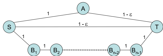
Figure 2: The most probable path may be long.
