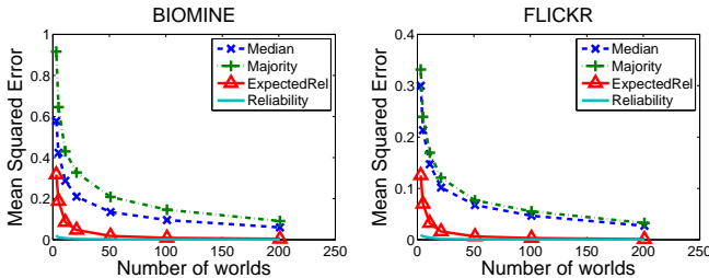
Figure 5: MSE vs. worlds. 200 worlds are enough.
