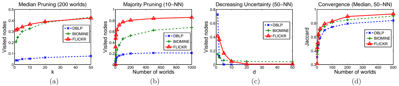
Figure 6: Number of visited nodes with respect to (a) k and (b) number of worlds. (c) Pruning efficiency vs. edge-probabilities; decreasing the uncertainty boosts the pruning power. (d) Convergence of the method.
